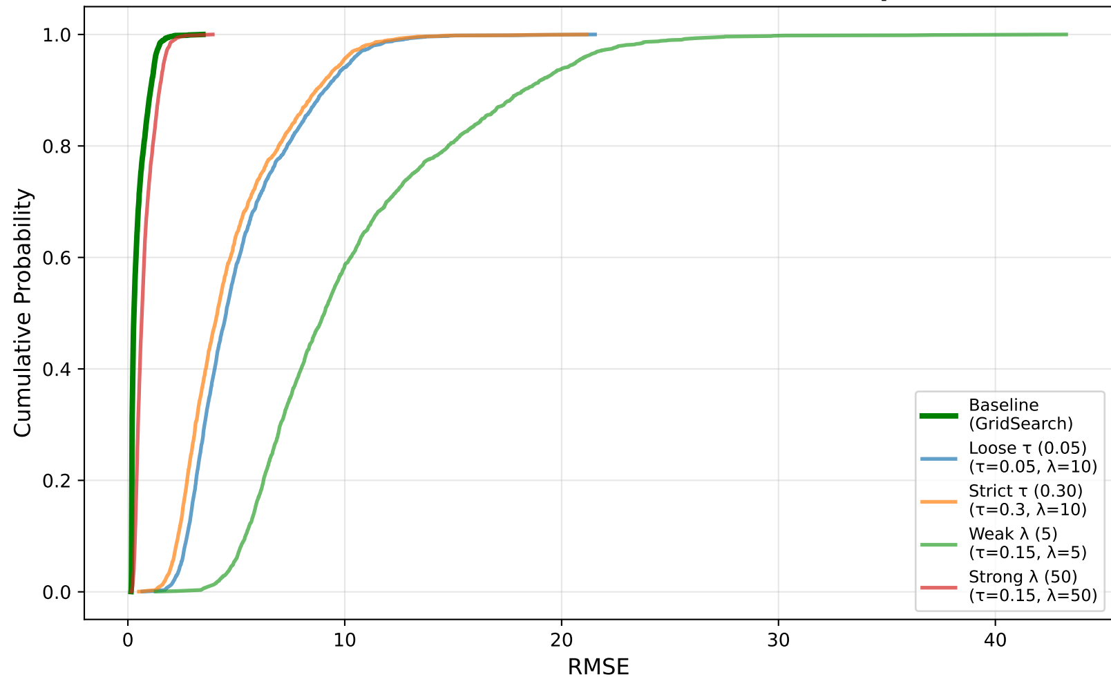
Cumulative Distribution Functions: RMSE Comparison
